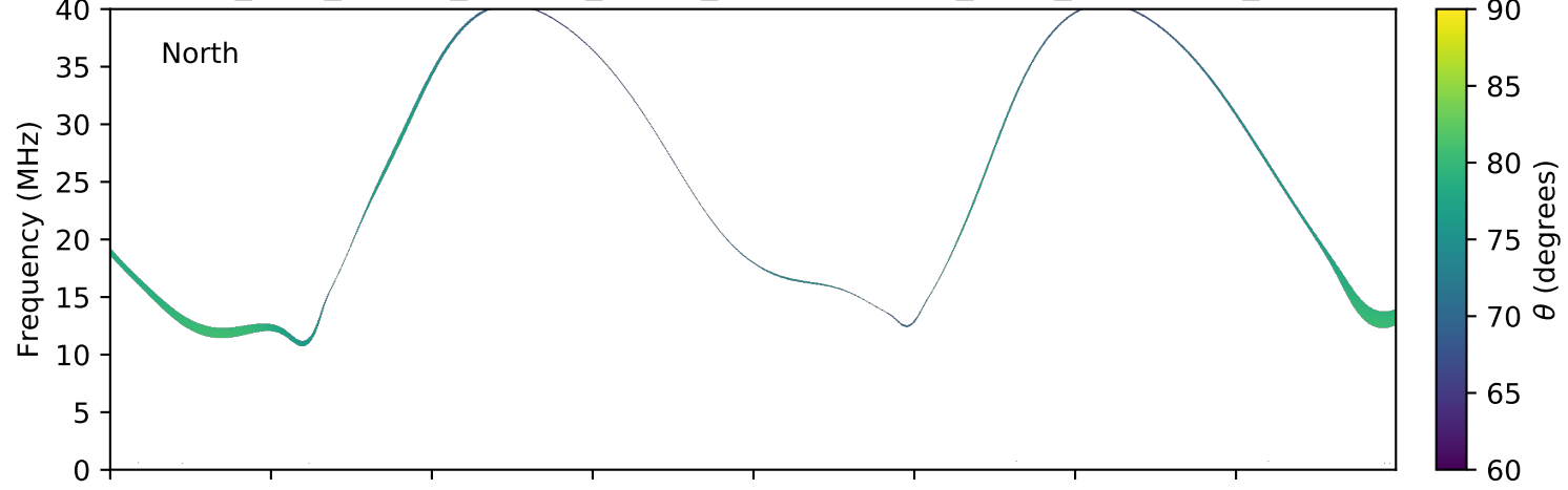
expres_juno_jupiter_europa_jrm09_lossc-wid1deg_3kev_20160918_v01.cdf
