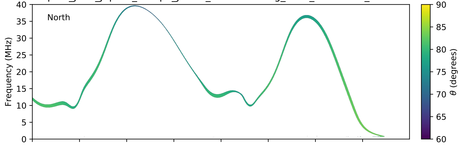
expres_juno_jupiter_europa_jrm09_lossc-wid1deg_3kev_20160904_v01.cdf
