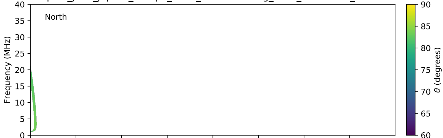
expres_juno_jupiter_europa_isaac_lossc-wid1deg_3kev_20160930_v01.cdf
