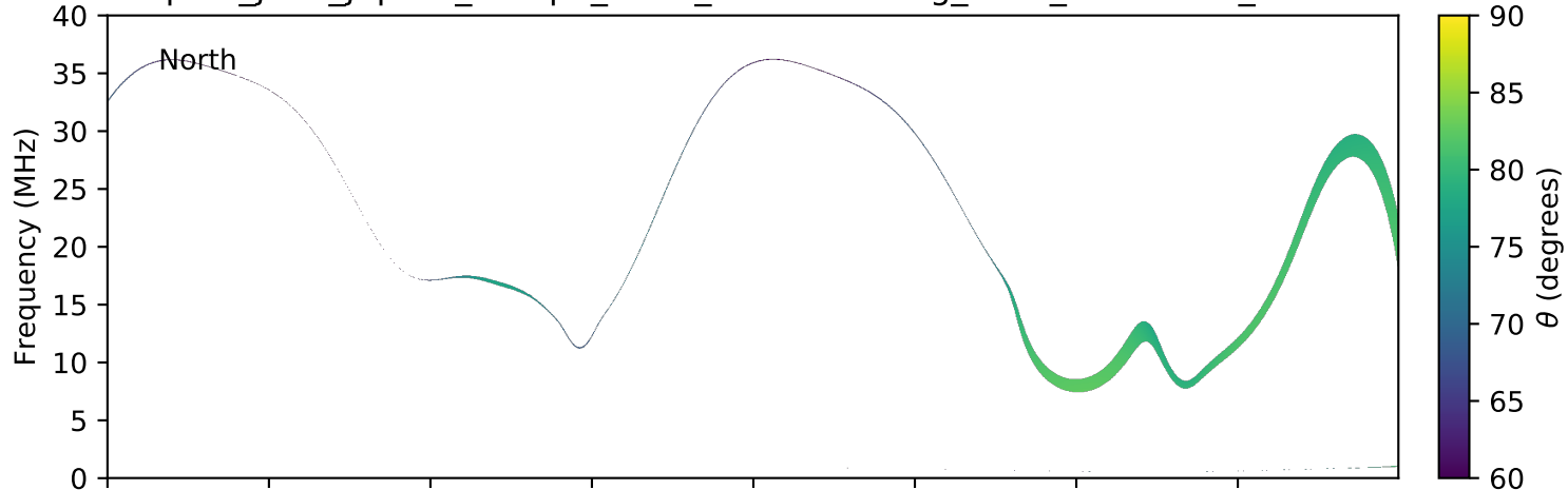
expres_juno_jupiter_europa_isaac_lossc-wid1deg_3kev_20160929_v01.cdf
