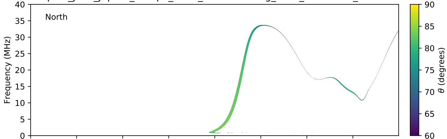
expres_juno_jupiter_europa_isaac_lossc-wid1deg_3kev_20160928_v01.cdf
