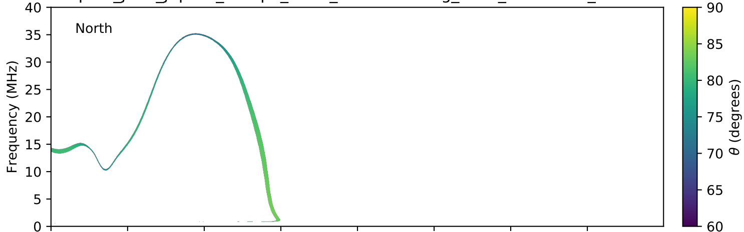
expres_juno_jupiter_europa_isaac_lossc-wid1deg_3kev_20160926_v01.cdf
