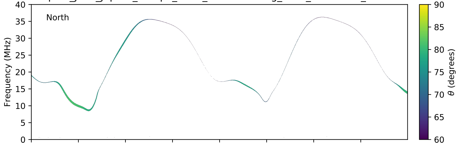
expres_juno_jupiter_europa_isaac_lossc-wid1deg_3kev_20160925_v01.cdf
