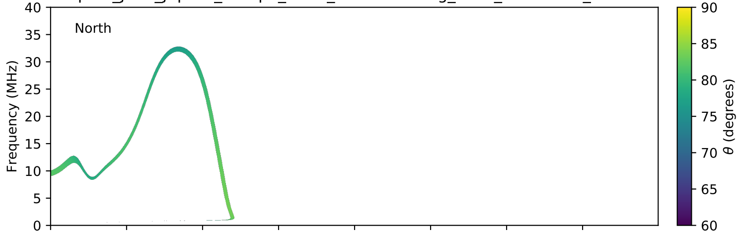
expres_juno_jupiter_europa_isaac_lossc-wid1deg_3kev_20160919_v01.cdf
