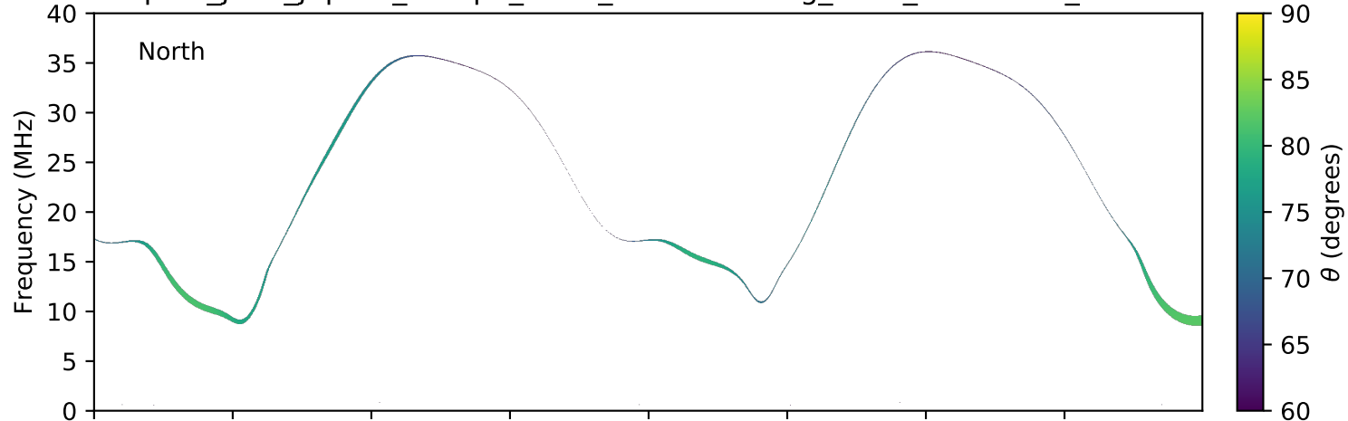
expres_juno_jupiter_europa_isaac_lossc-wid1deg_3kev_20160918_v01.cdf
