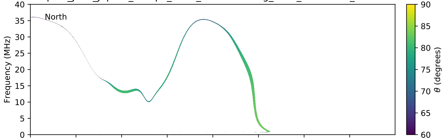
expres_juno_jupiter_europa_isaac_lossc-wid1deg_3kev_20160915_v01.cdf
