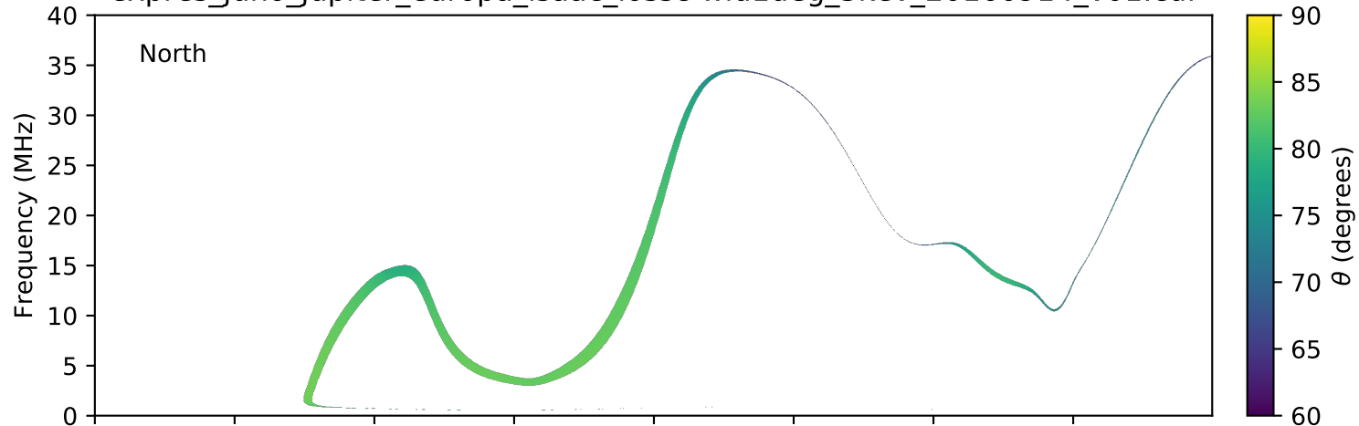
expres_juno_jupiter_europa_isaac_lossc-wid1deg_3kev_20160914_v01.cdf
