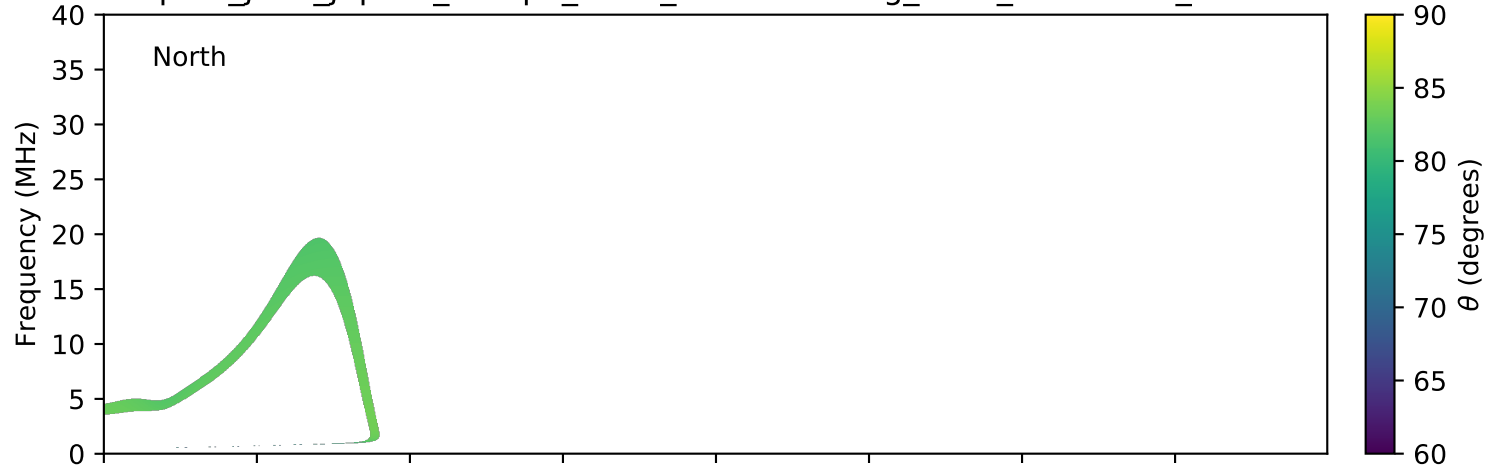
expres_juno_jupiter_europa_isaac_lossc-wid1deg_3kev_20160912_v01.cdf
