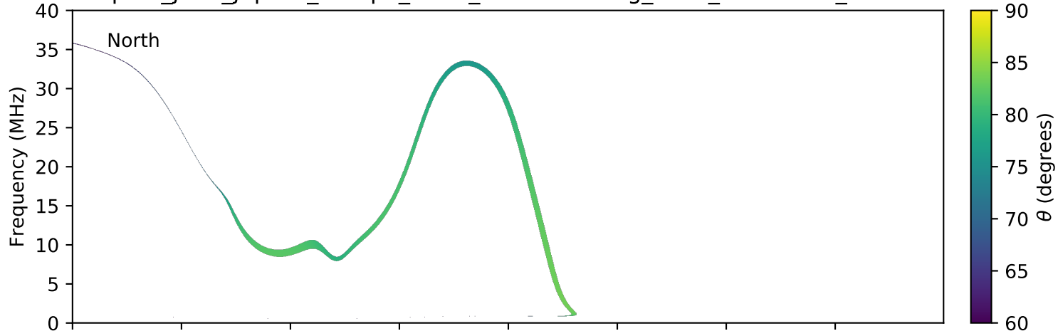
expres_juno_jupiter_europa_isaac_lossc-wid1deg_3kev_20160908_v01.cdf
