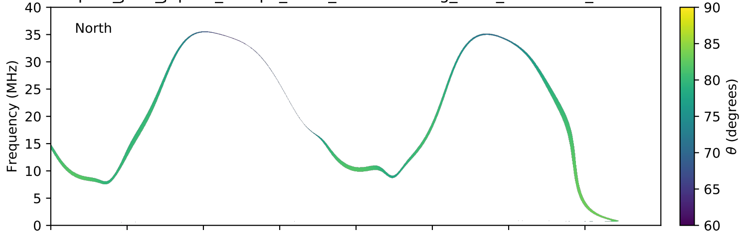
expres_juno_jupiter_europa_isaac_lossc-wid1deg_3kev_20160904_v01.cdf
