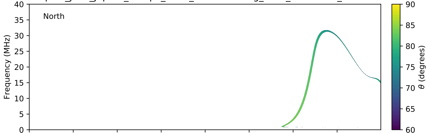
expres_juno_jupiter_europa_isaac_lossc-wid1deg_3kev_20160903_v01.cdf
