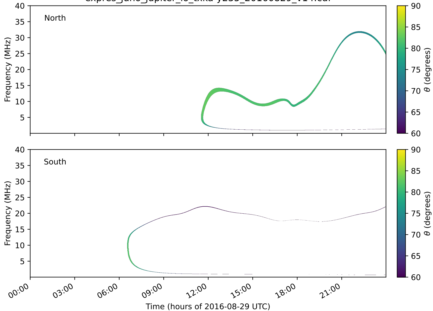
expres_juno_jupiter_io_txka-y235_20160829_v14.cdf
