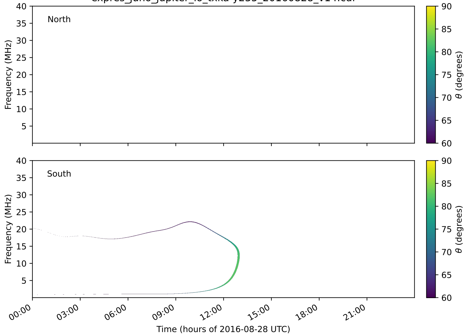
expres_juno_jupiter_io_txka-y235_20160828_v14.cdf
