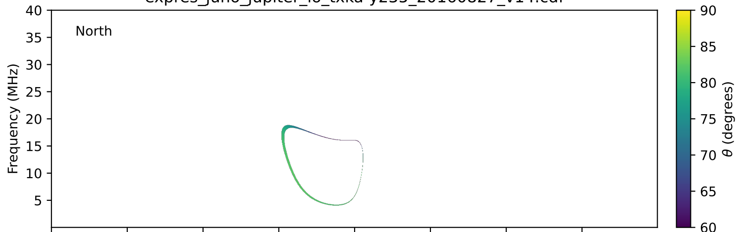
expres_juno_jupiter_io_txka-y235_20160827_v14.cdf
