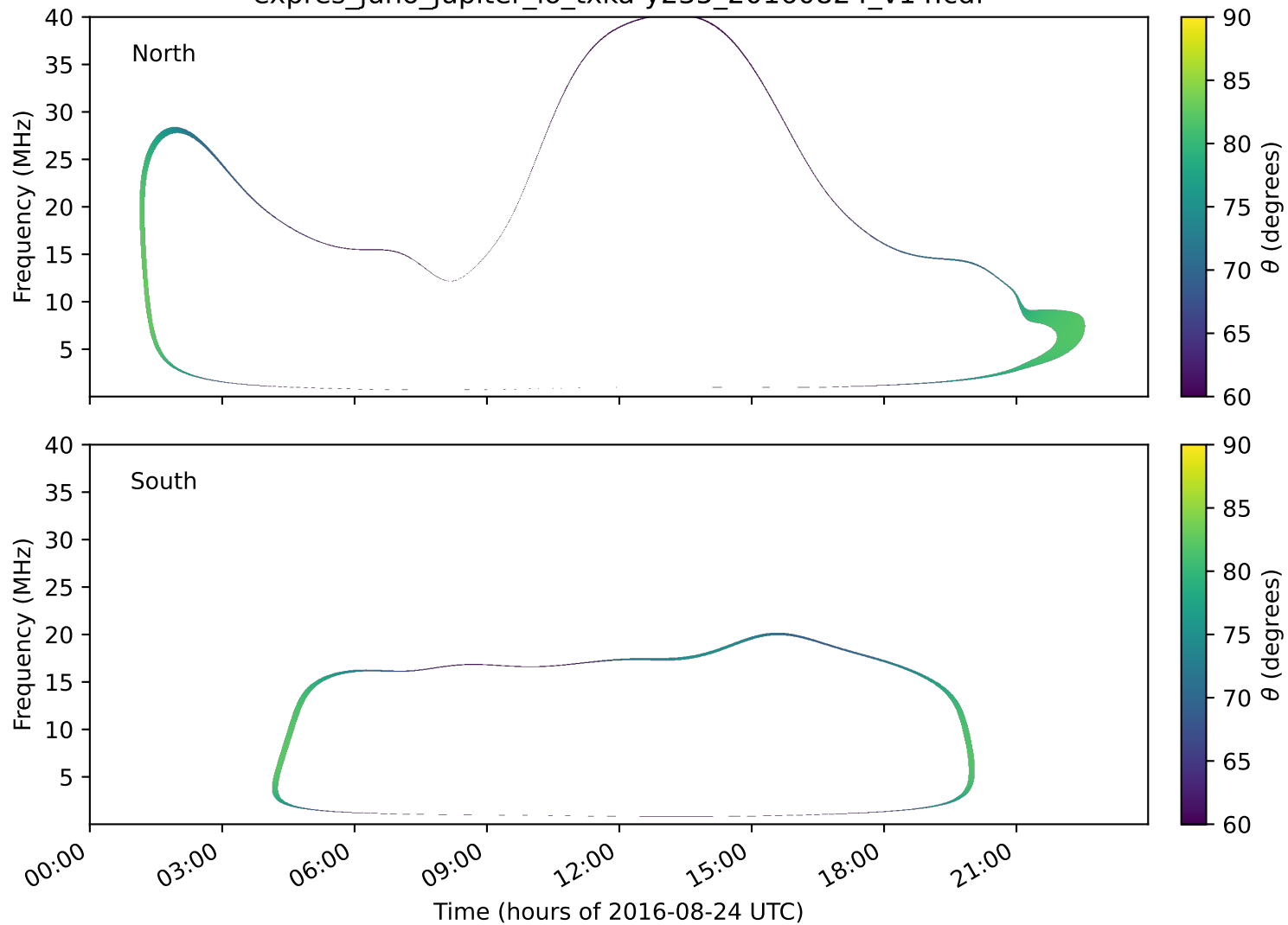
expres_juno_jupiter_io_txka-y235_20160824_v14.cdf
