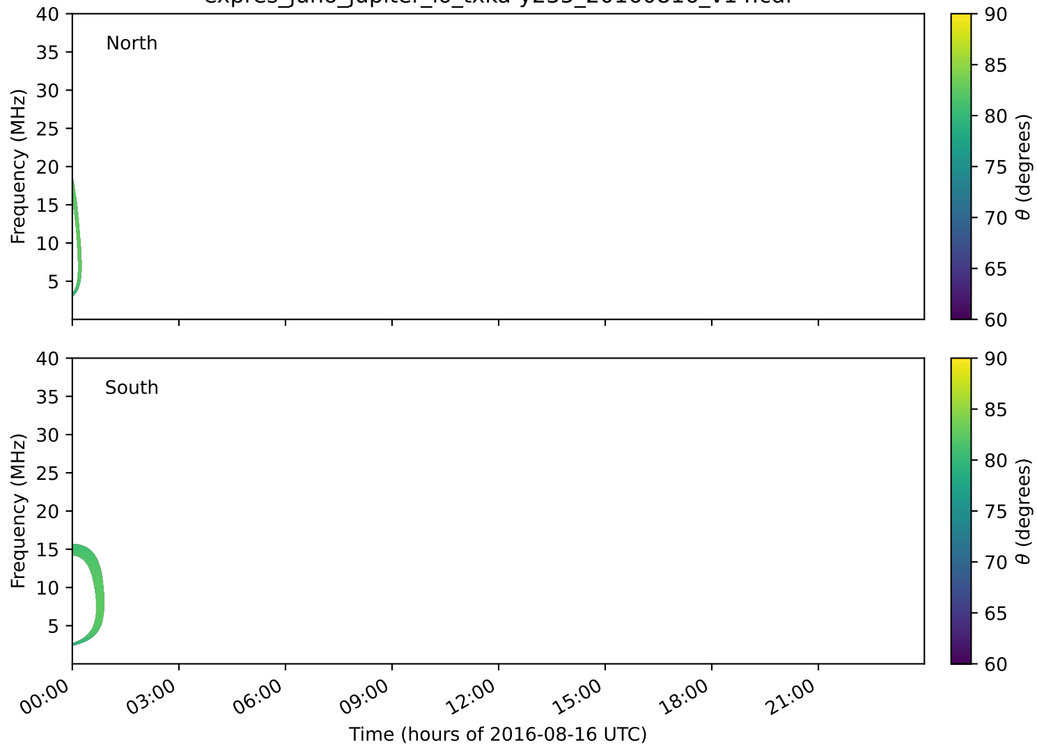
expres_juno_jupiter_io_txka-y235_20160816_v14.cdf
