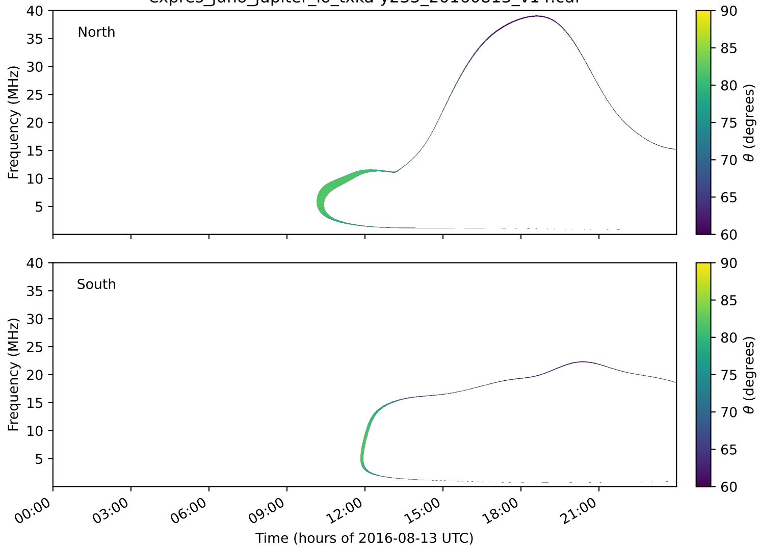
expres_juno_jupiter_io_txka-y235_20160813_v14.cdf
