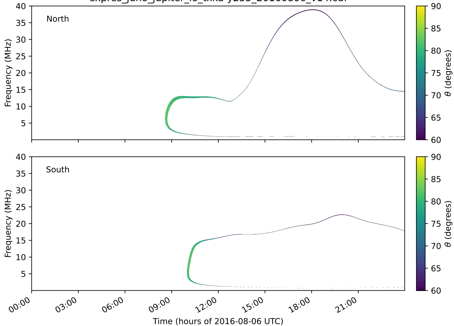
expres_juno_jupiter_io_txka-y235_20160806_v14.cdf
