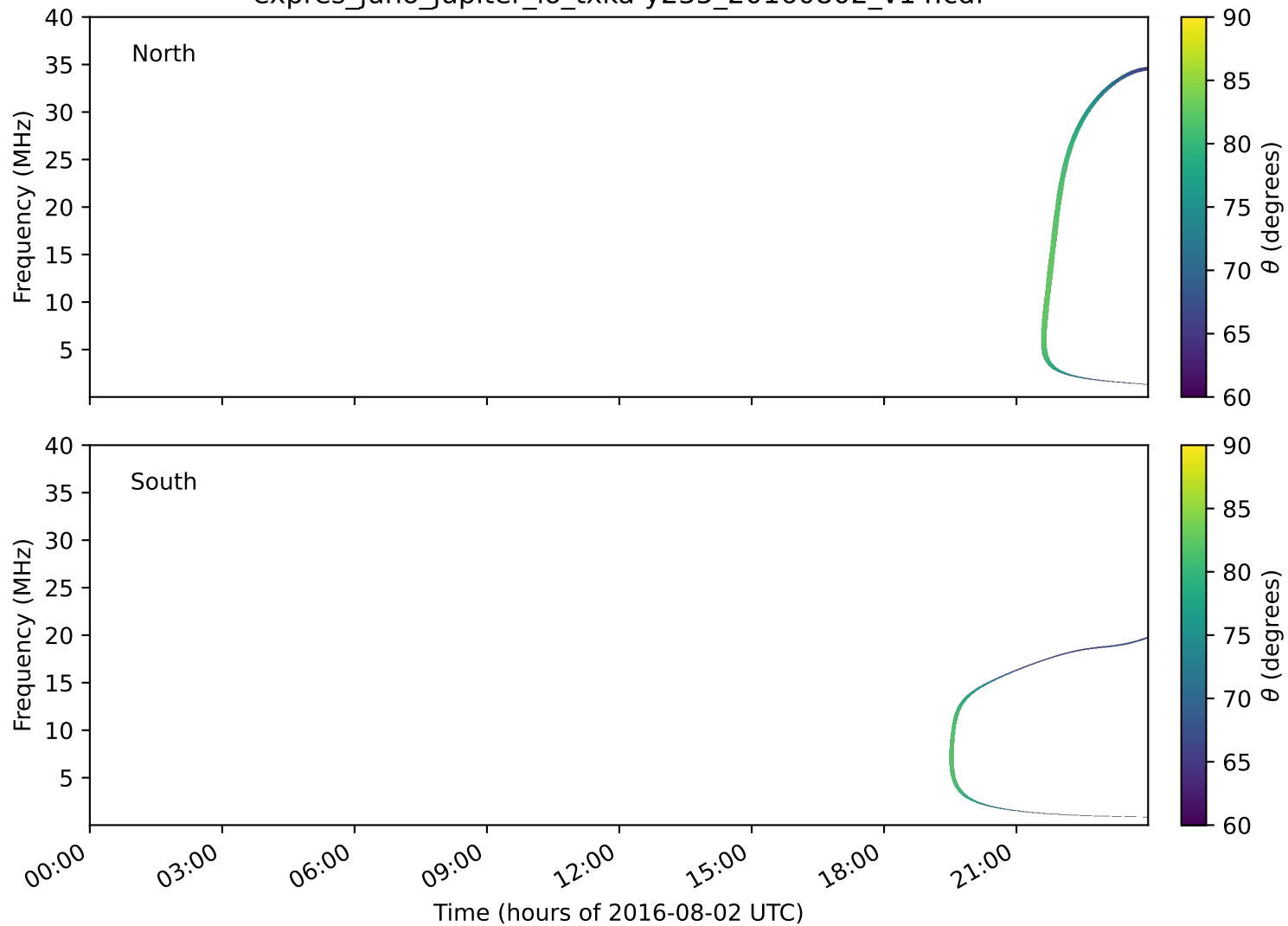
expres_juno_jupiter_io_txka-y235_20160802_v14.cdf
