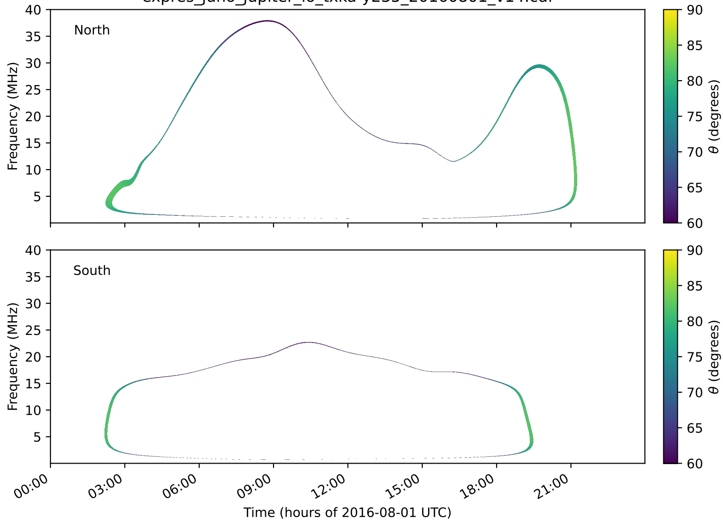
expres_juno_jupiter_io_txka-y235_20160801_v14.cdf
