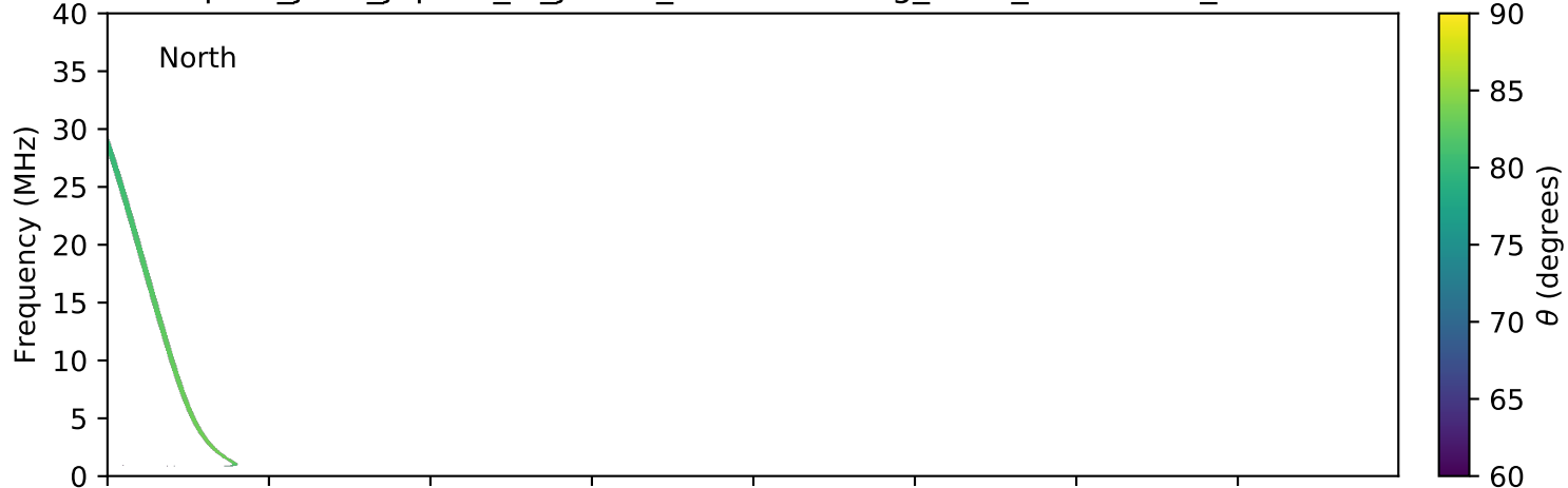
expres_juno_jupiter_io_jrm09_lossc-wid1deg_3kev_20160830_v01.cdf
