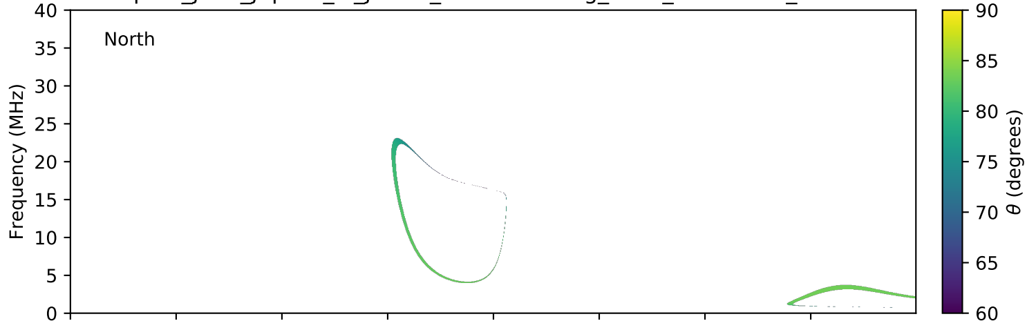
expres_juno_jupiter_io_jrm09_lossc-wid1deg_3kev_20160827_v01.cdf
