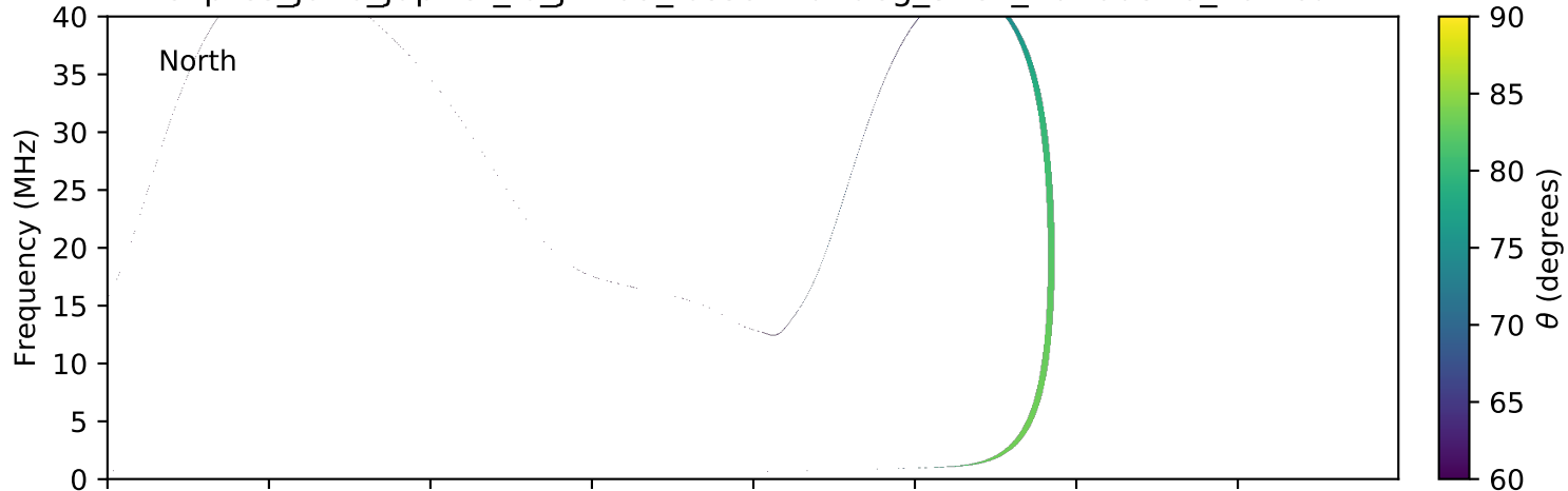
expres_juno_jupiter_io_jrm09_lossc-wid1deg_3kev_20160826_v01.cdf
