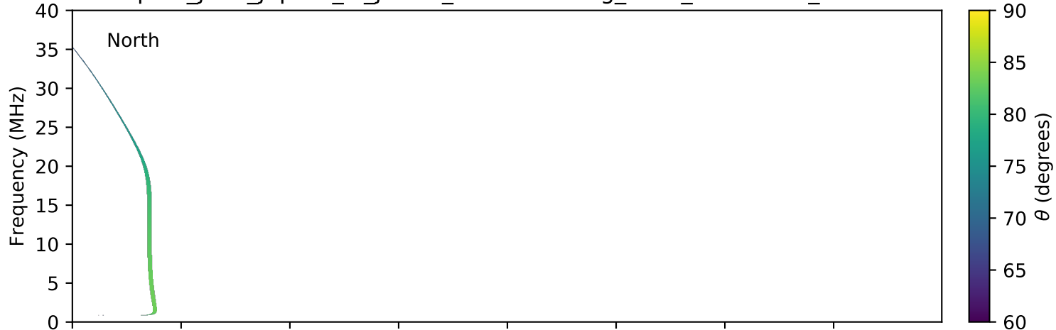
expres_juno_jupiter_io_jrm09_lossc-wid1deg_3kev_20160823_v01.cdf
