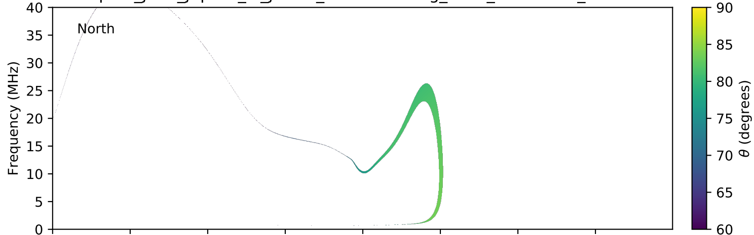
expres_juno_jupiter_io_jrm09_lossc-wid1deg_3kev_20160819_v01.cdf
