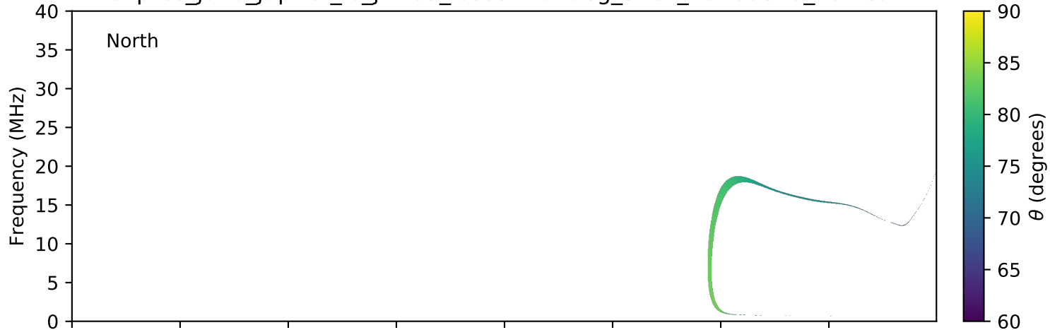
expres_juno_jupiter_io_jrm09_lossc-wid1deg_3kev_20160818_v01.cdf
