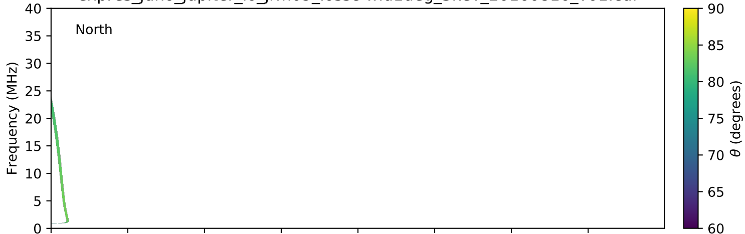
expres_juno_jupiter_io_jrm09_lossc-wid1deg_3kev_20160816_v01.cdf
