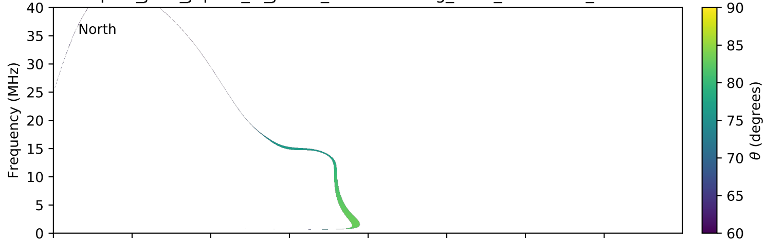
expres_juno_jupiter_io_jrm09_lossc-wid1deg_3kev_20160812_v01.cdf
