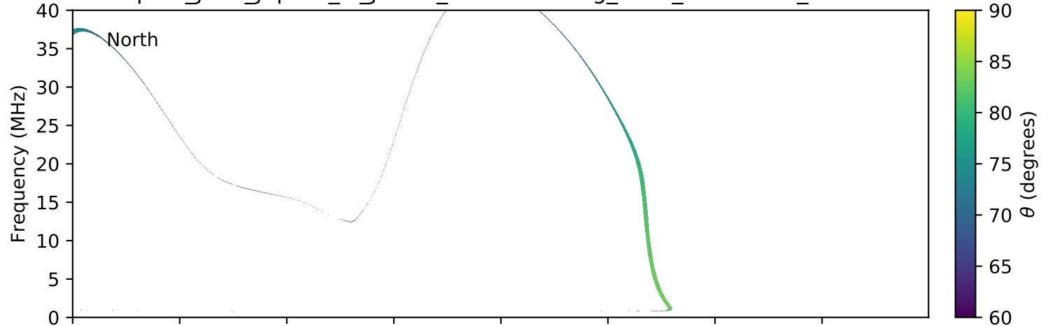
expres_juno_jupiter_io_jrm09_lossc-wid1deg_3kev_20160810_v01.cdf
