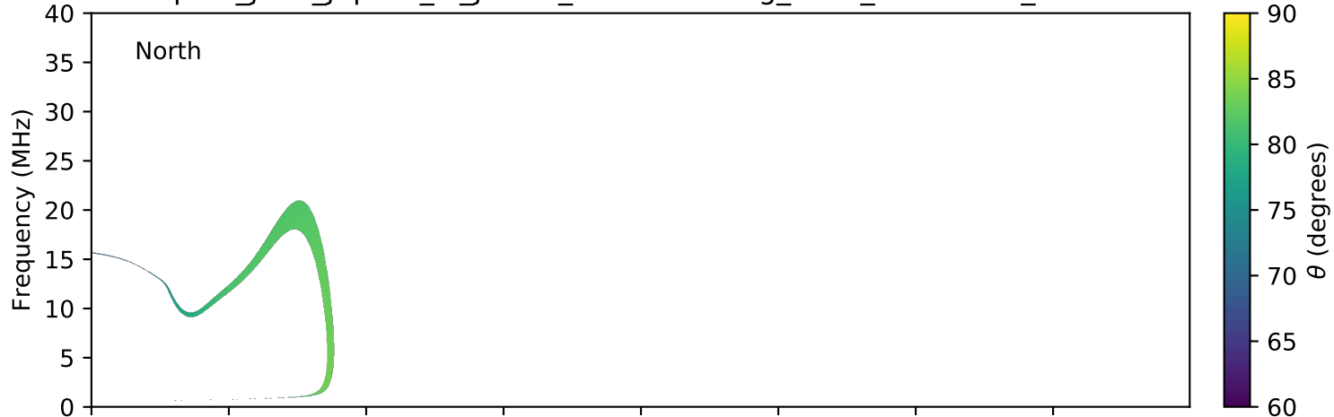
expres_juno_jupiter_io_jrm09_lossc-wid1deg_3kev_20160807_v01.cdf
