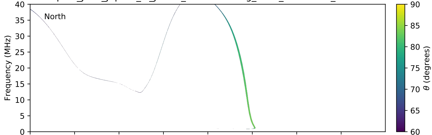
expres_juno_jupiter_io_jrm09_lossc-wid1deg_3kev_20160803_v01.cdf
