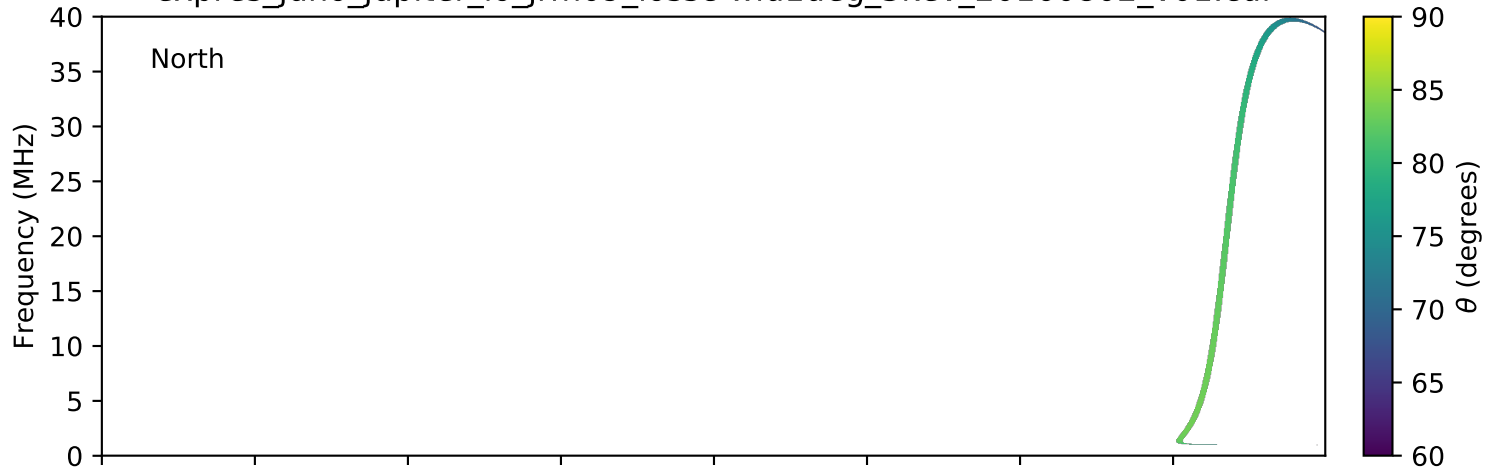
expres_juno_jupiter_io_jrm09_lossc-wid1deg_3kev_20160802_v01.cdf
