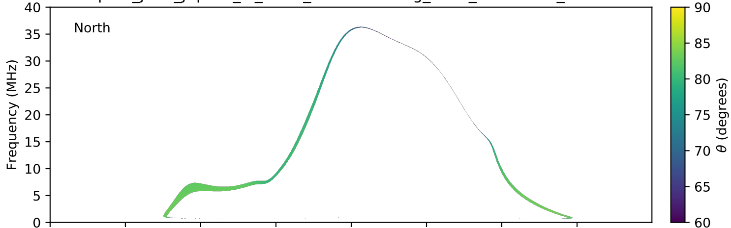
expres_juno_jupiter_io_isaac_lossc-wid1deg_3kev_20160831_v01.cdf
