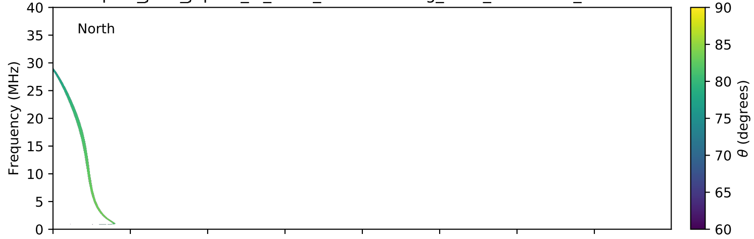
expres_juno_jupiter_io_isaac_lossc-wid1deg_3kev_20160830_v01.cdf
