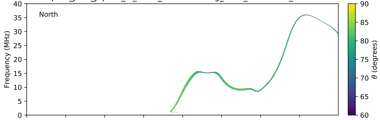
expres_juno_jupiter_io_isaac_lossc-wid1deg_3kev_20160829_v01.cdf
