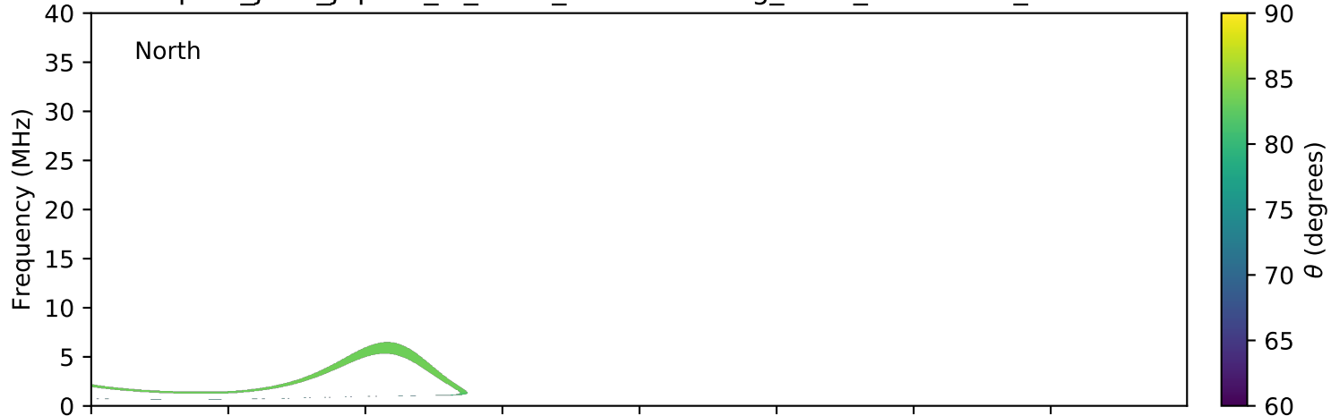
expres_juno_jupiter_io_isaac_lossc-wid1deg_3kev_20160828_v01.cdf
