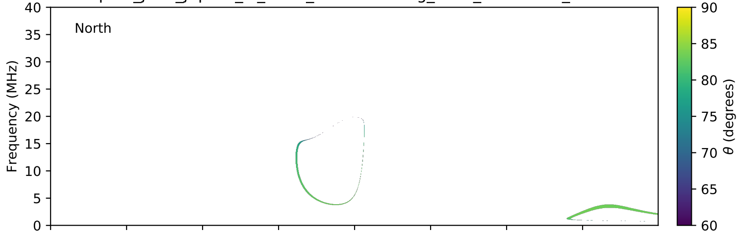
expres_juno_jupiter_io_isaac_lossc-wid1deg_3kev_20160827_v01.cdf
