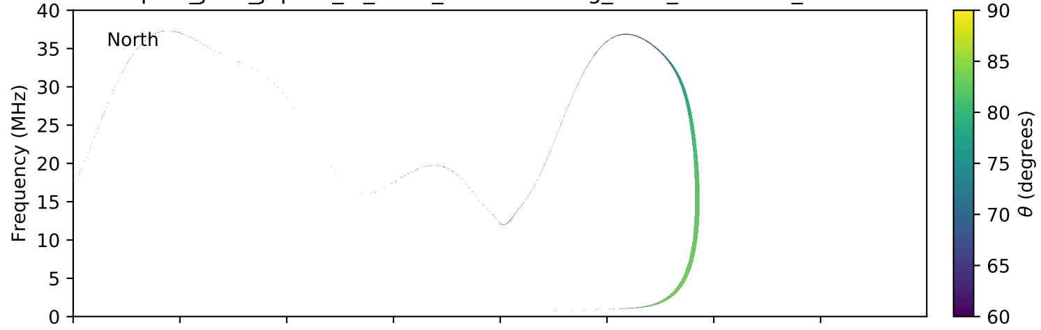
expres_juno_jupiter_io_isaac_lossc-wid1deg_3kev_20160826_v01.cdf
