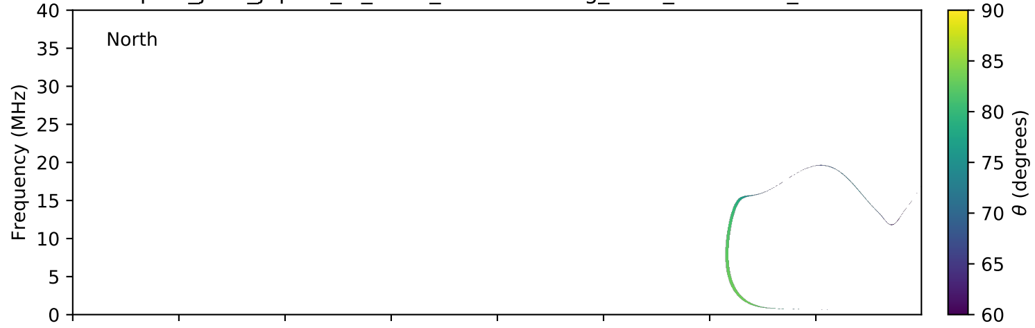
expres_juno_jupiter_io_isaac_lossc-wid1deg_3kev_20160825_v01.cdf
