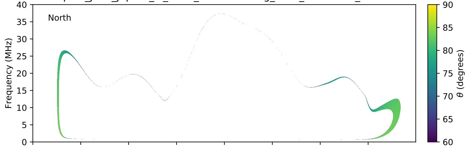
expres_juno_jupiter_io_isaac_lossc-wid1deg_3kev_20160824_v01.cdf
