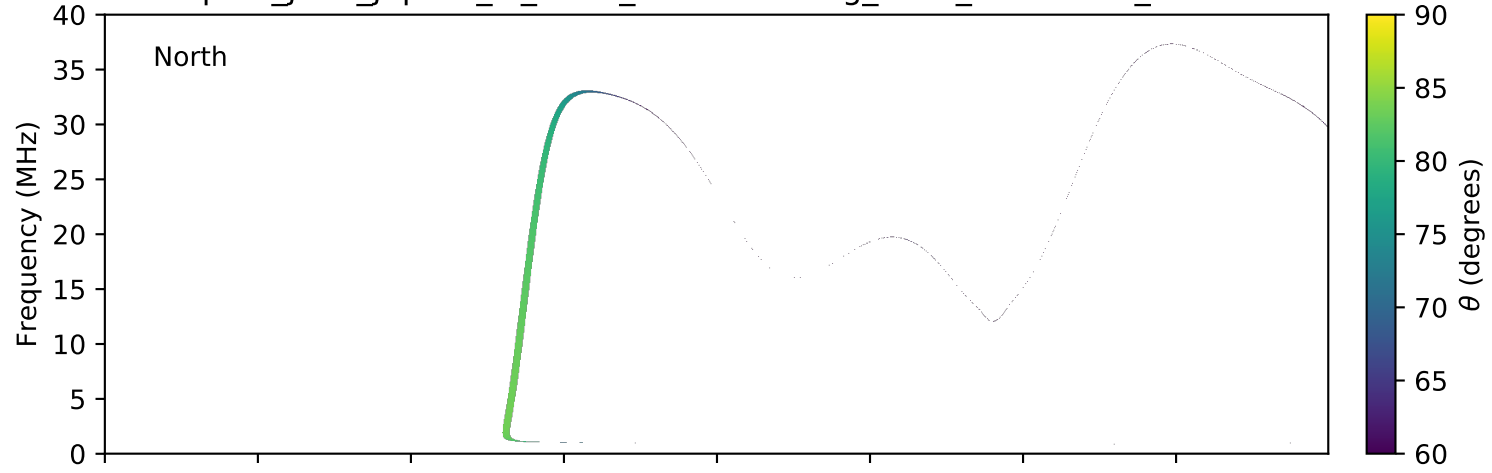
expres_juno_jupiter_io_isaac_lossc-wid1deg_3kev_20160822_v01.cdf
