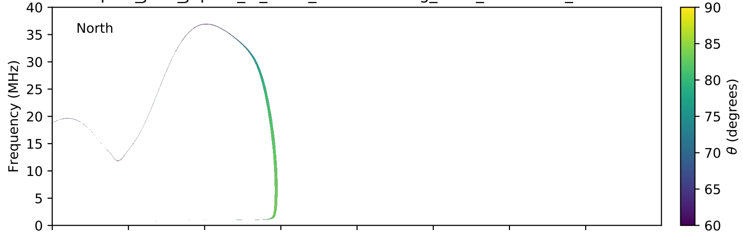
expres_juno_jupiter_io_isaac_lossc-wid1deg_3kev_20160821_v01.cdf
