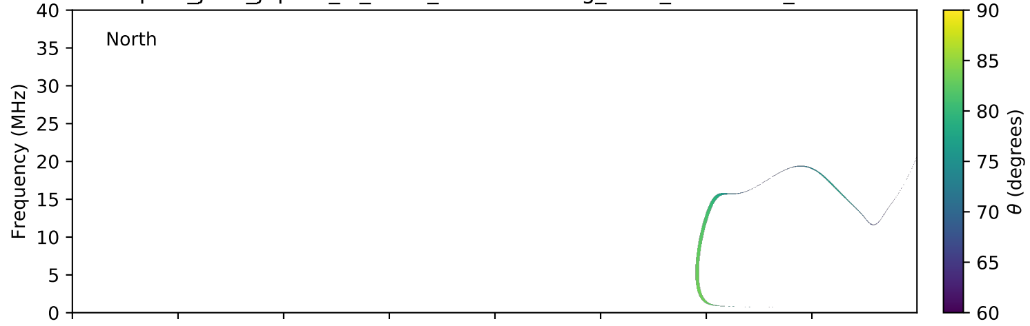
expres_juno_jupiter_io_isaac_lossc-wid1deg_3kev_20160818_v01.cdf
