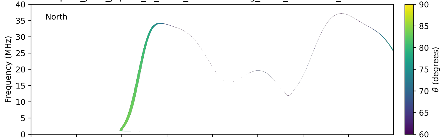
expres_juno_jupiter_io_isaac_lossc-wid1deg_3kev_20160815_v01.cdf
