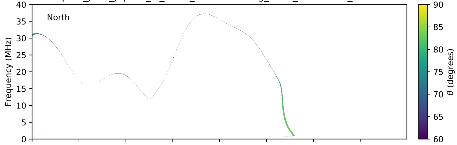
expres_juno_jupiter_io_isaac_lossc-wid1deg_3kev_20160810_v01.cdf
