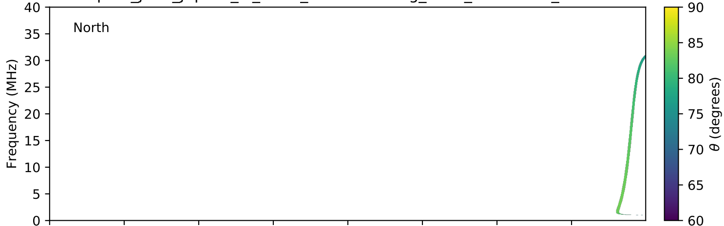
expres_juno_jupiter_io_isaac_lossc-wid1deg_3kev_20160809_v01.cdf
